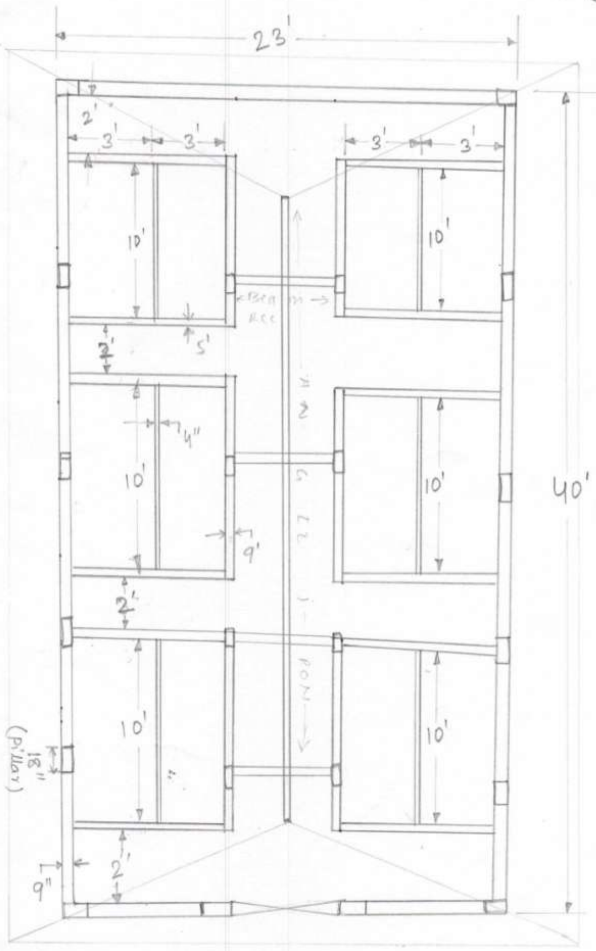
Top View
